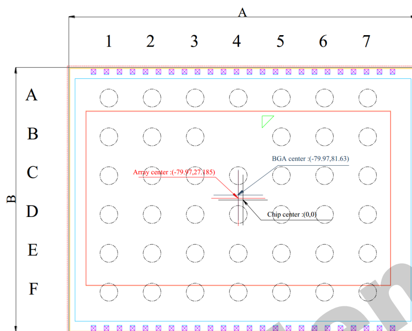
GC4663 Package diagram (Top View Image Side unit: \mu\text{m} )
