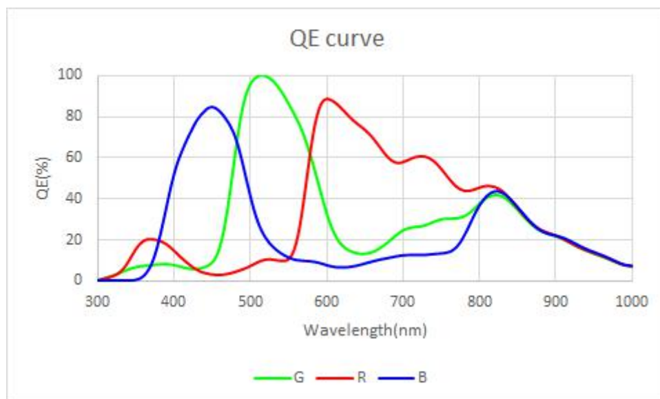
图 4-1 QE Curve
