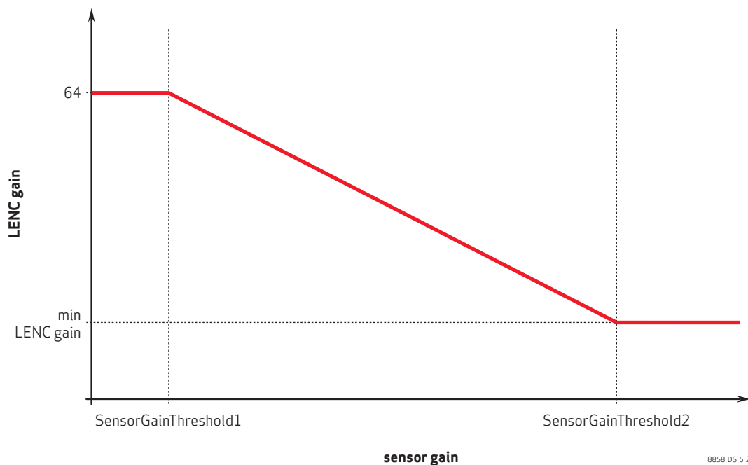
figure 5-3 luminance compensation level calculation
