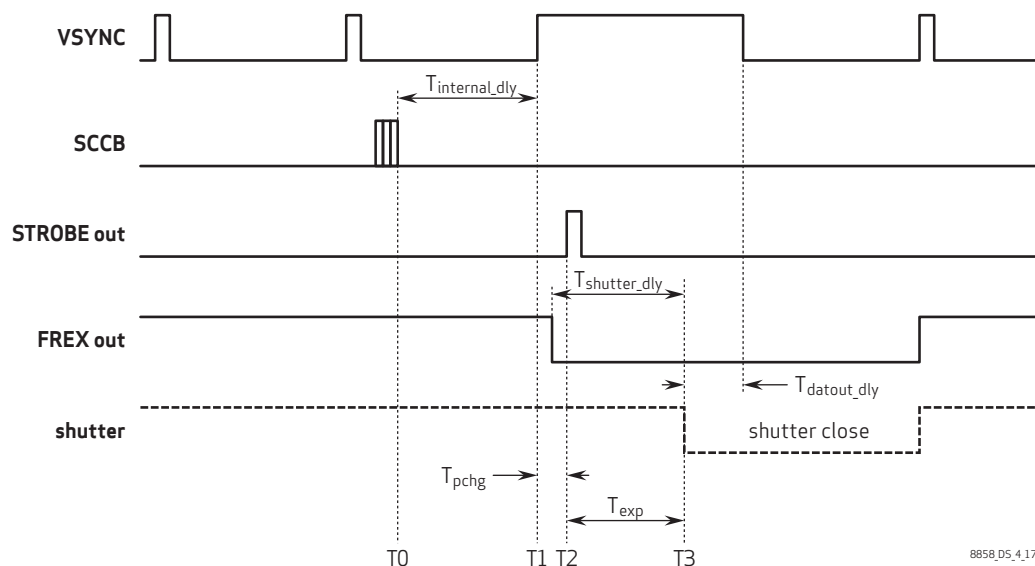
figure 4-16 FREX mode 2 (shutter delay &gt; 0) timing diagram
