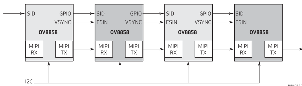
figure 2-21 MIPI daisy chain diagram
