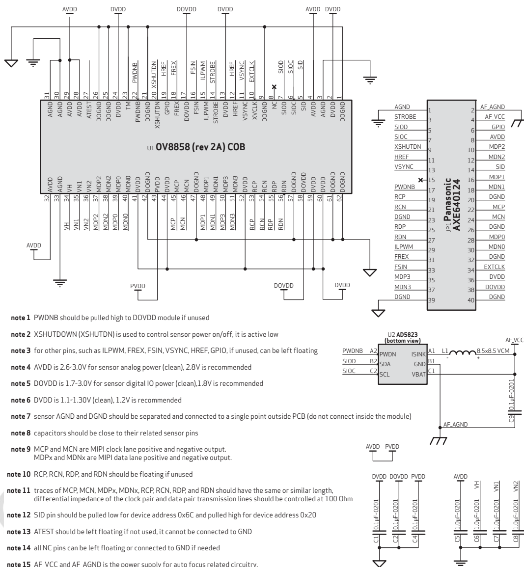
figure 2-2 OV8858 reference schematic
