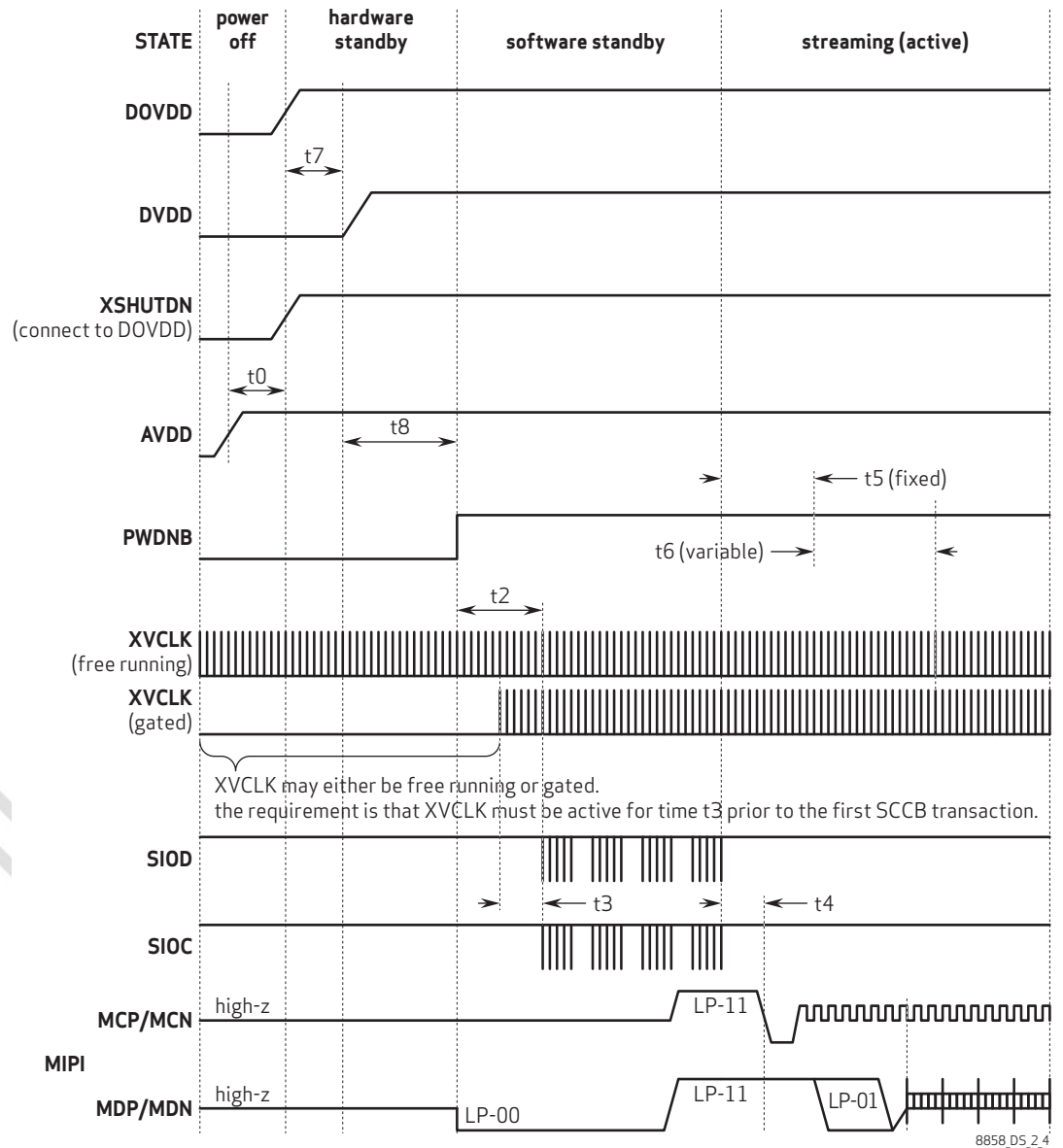
figure 2-4 power up sequence (case 2)
