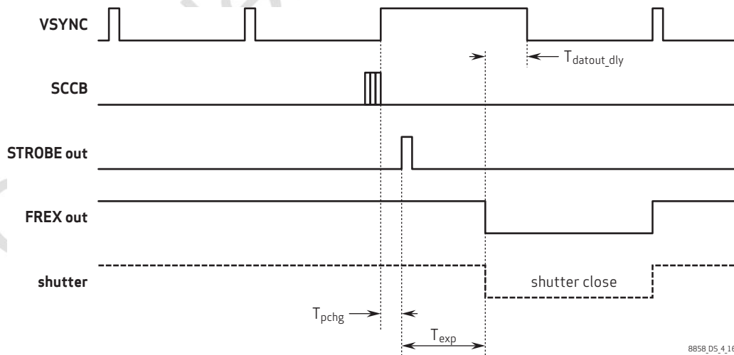
figure 4-15 FREX mode 2 (shutter delay = 0) timing diagram
