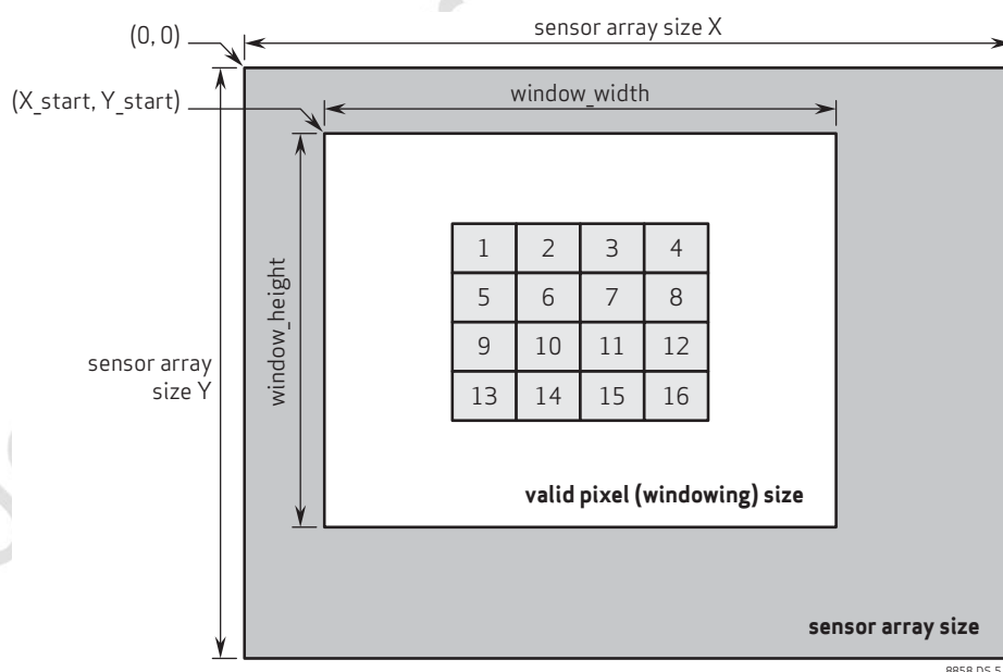
figure 5-1 average-based window definition
