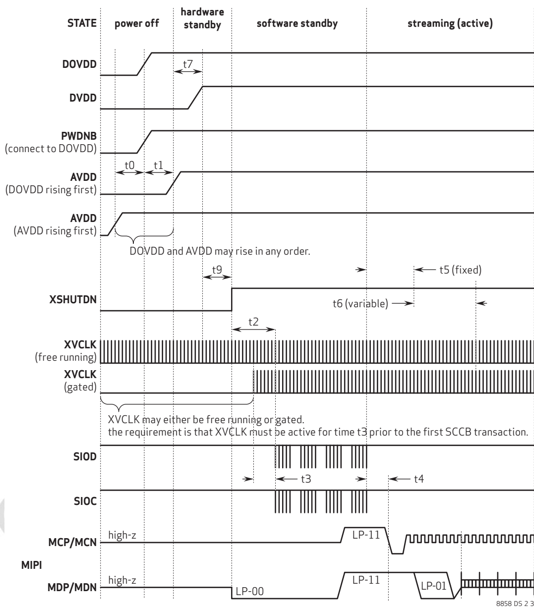
figure 2-3 power up sequence (case 1)
