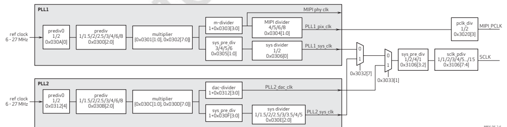
figure 2-6 clock scheme
