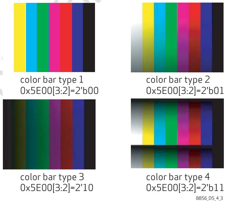
figure 4-3 color bar types
