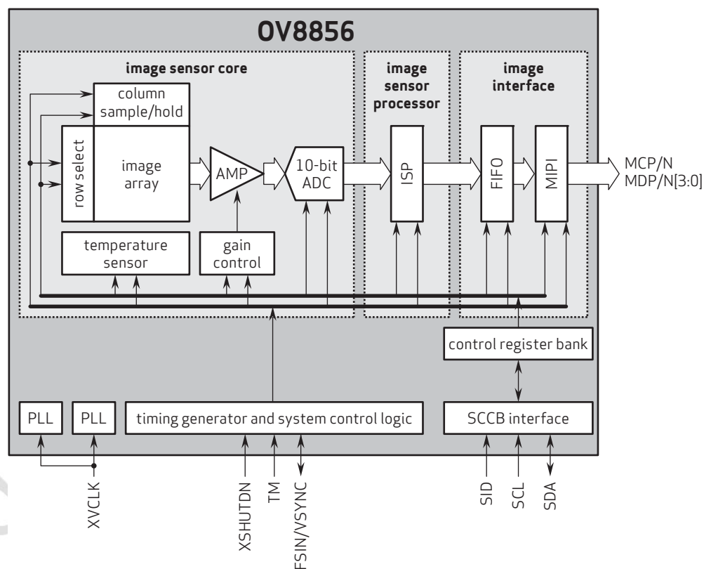
figure 2-1 OV8856 block diagram
