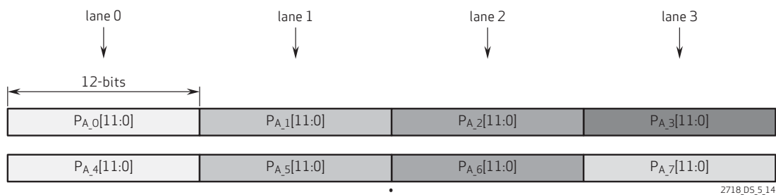
figure 5-14 12b compressed combined DCG HDR diagram
