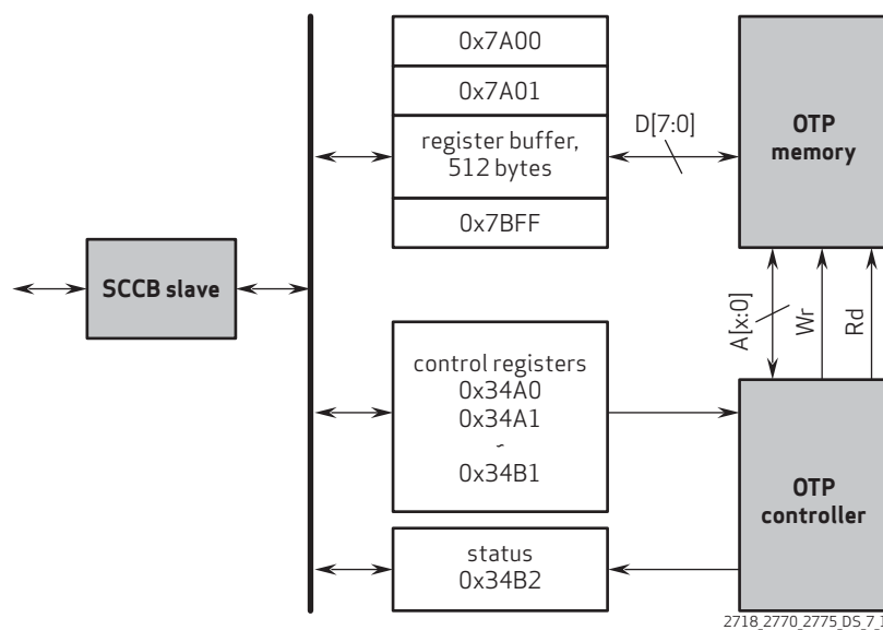
figure 7-1 OTP memory diagram
