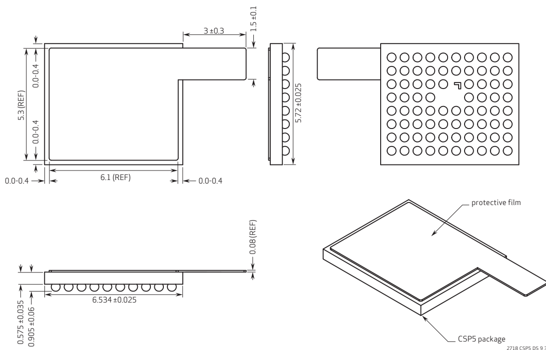
figure 9-3 protective film specifications
