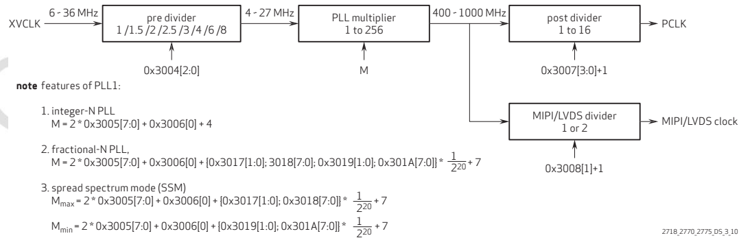
figure 3-9 PLL1 control diagram
