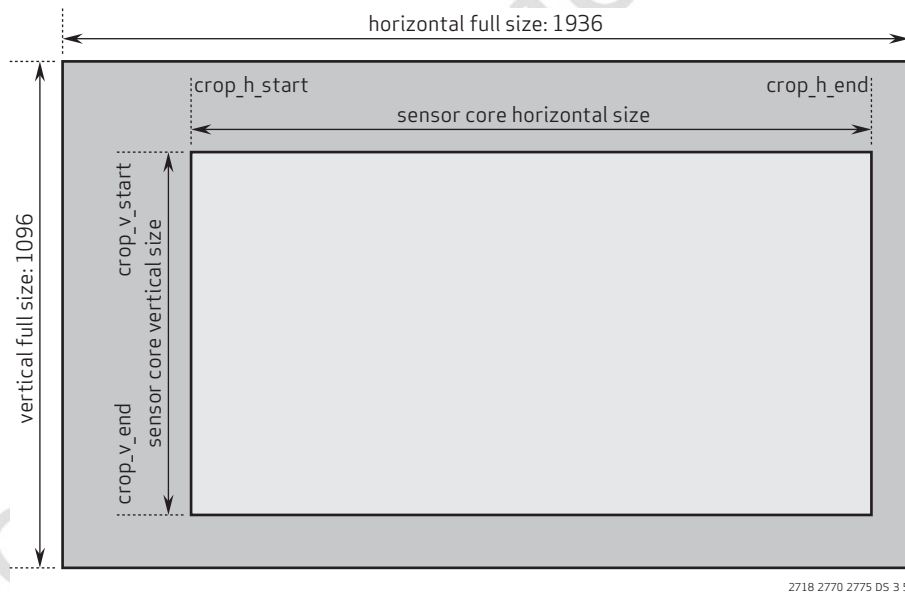
figure 3-4 pixel array access diagram
