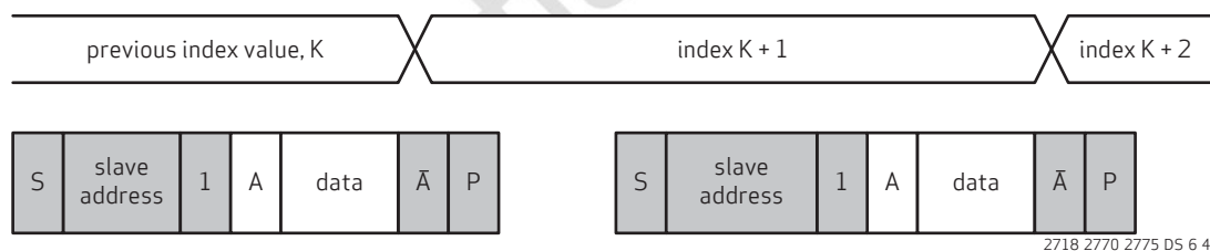
figure 6-4 SCCB single read from current location
