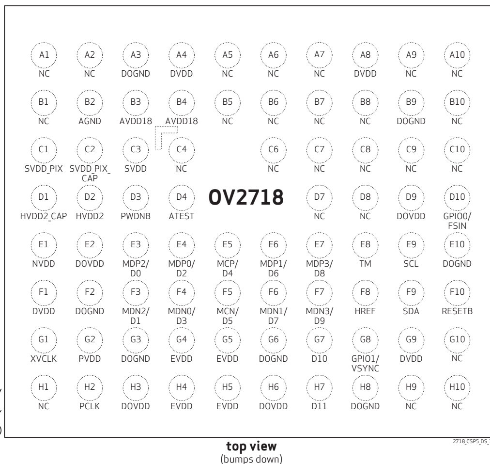
figure 1-1 pin diagram
