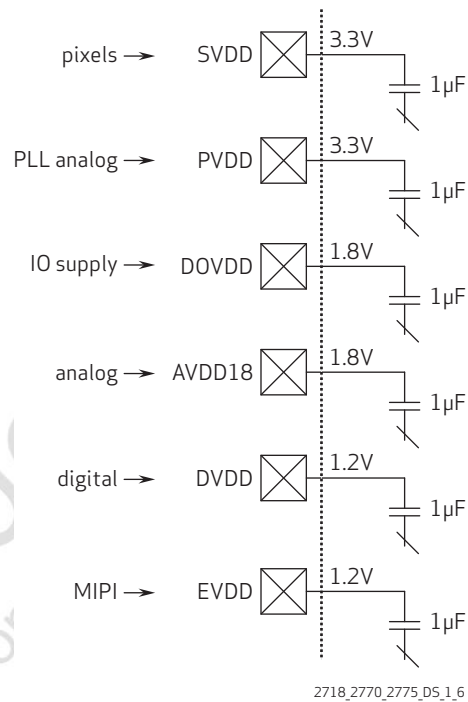
figure 1-4 OV2718 power supplies and recommended external decoupling
