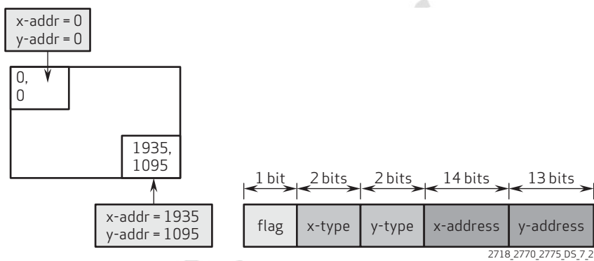
figure 7-2 defect pixel address description
