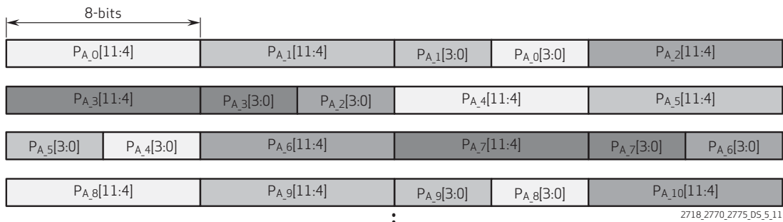
figure 5-6 12b linear mode diagram
