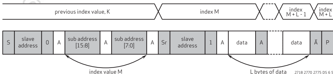
figure 6-5 SCCB sequential read from random location
