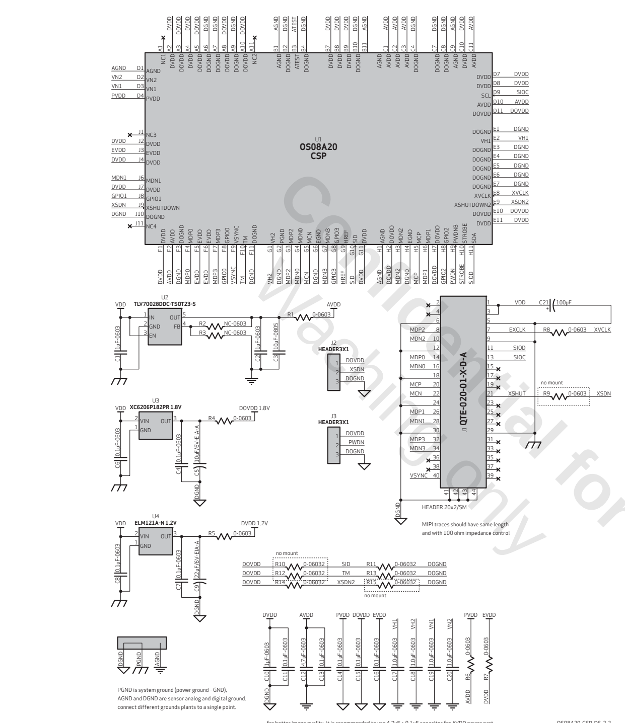
figure 2-2 OS08A20 reference schematic
