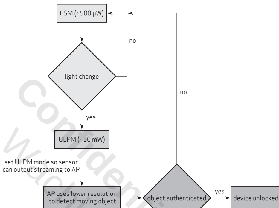
figure 4-14 low power mode example
