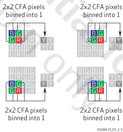
figure 3-3 example of 2x2 mono binning
