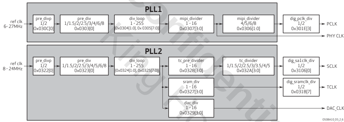
figure 2-6 clock scheme
