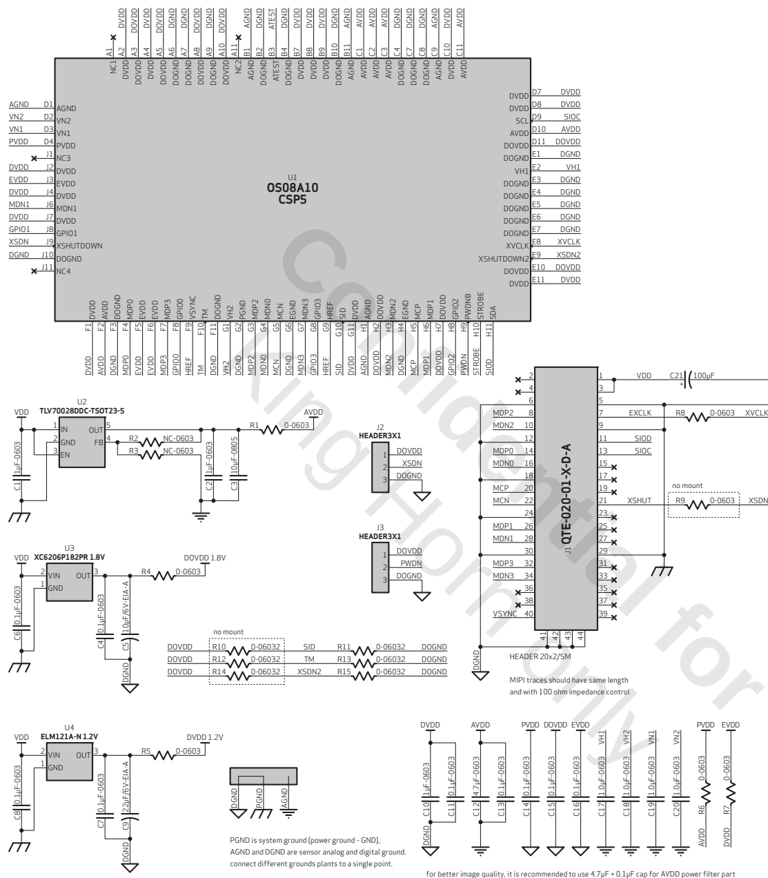
figure 2-2 OS08A10 reference schematic
