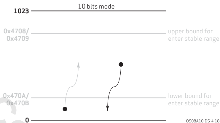
figure 4-18 mode 2 stable range diagram
