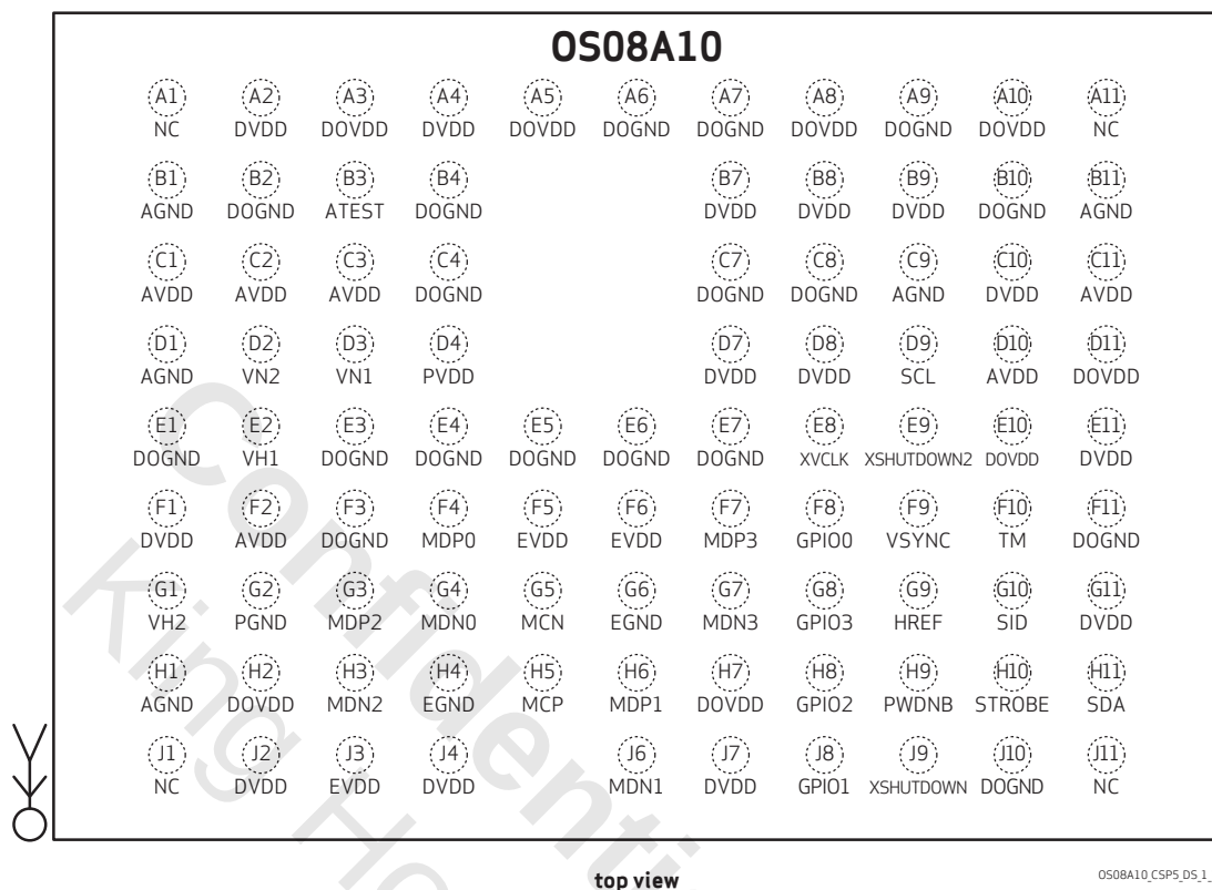
figure 1-1 pin diagram
