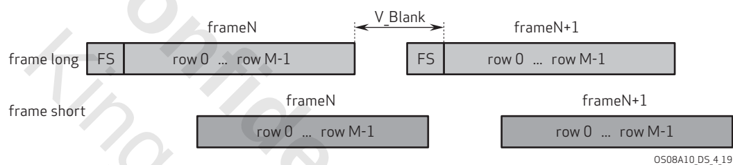
figure 4-19 set staggered HDR
