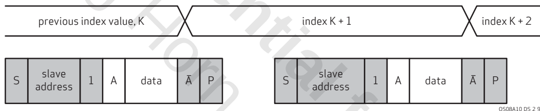
figure 2-9 SCCB single read from current location
