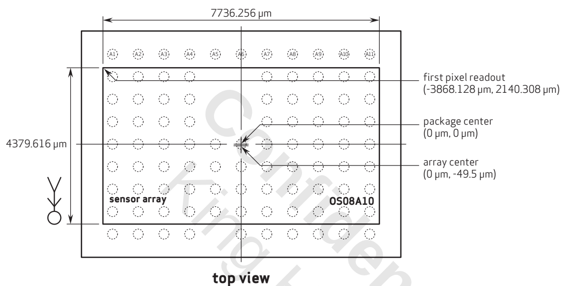
figure 9-1 sensor array center
