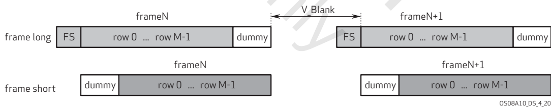
figure 4-20 set staggered HDR with no VC
