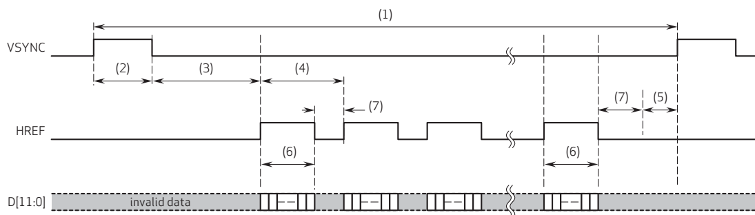
figure 5-5 DVP timing diagram
