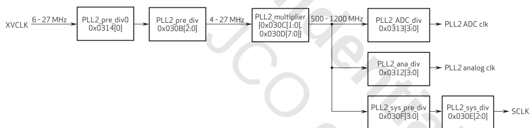
figure 3-6 PLL2 clock diagram
