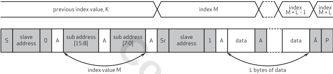
figure 6-4 SCCB sequential read from random location
