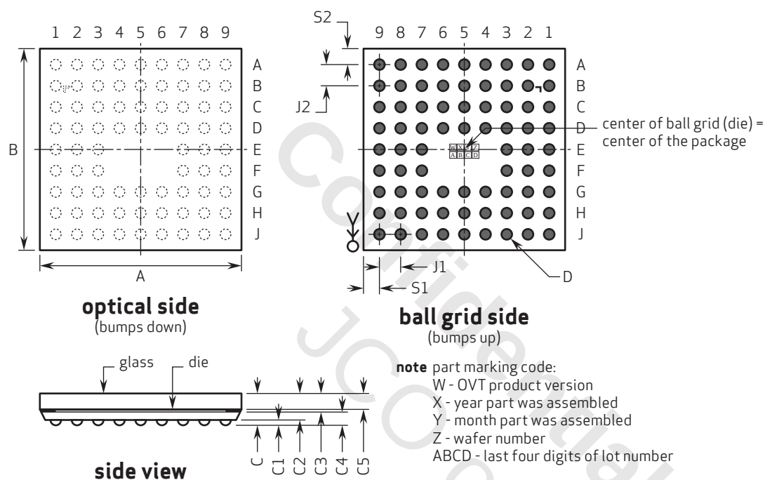
figure 9-1 package specifications
