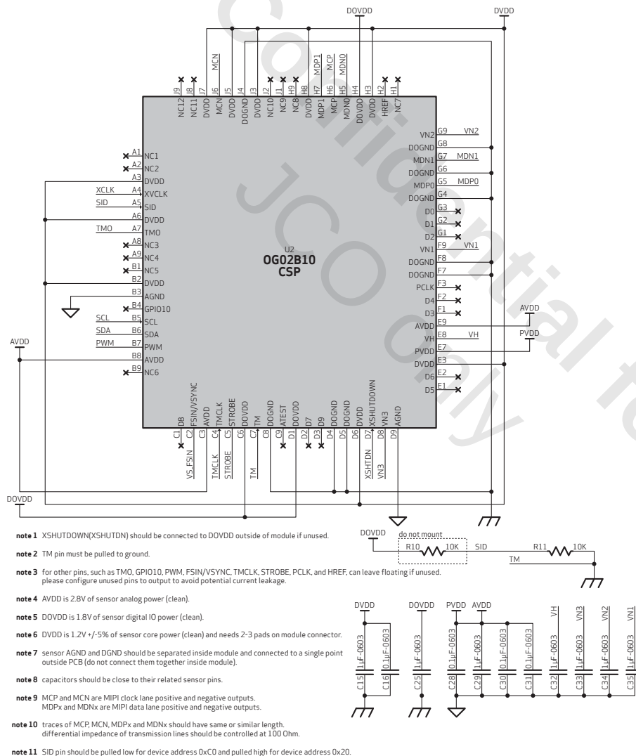
figure 1-2 OG02B10 MIPI reference design schematic
