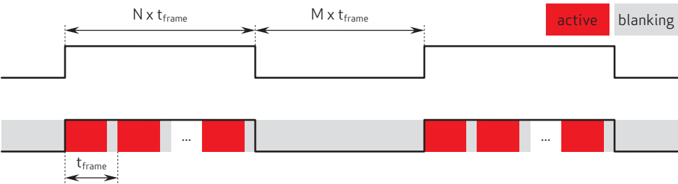
figure 3-10 low frame rate mode timing
