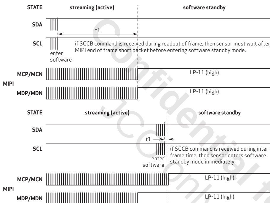
figure 1-6 standby sequence
