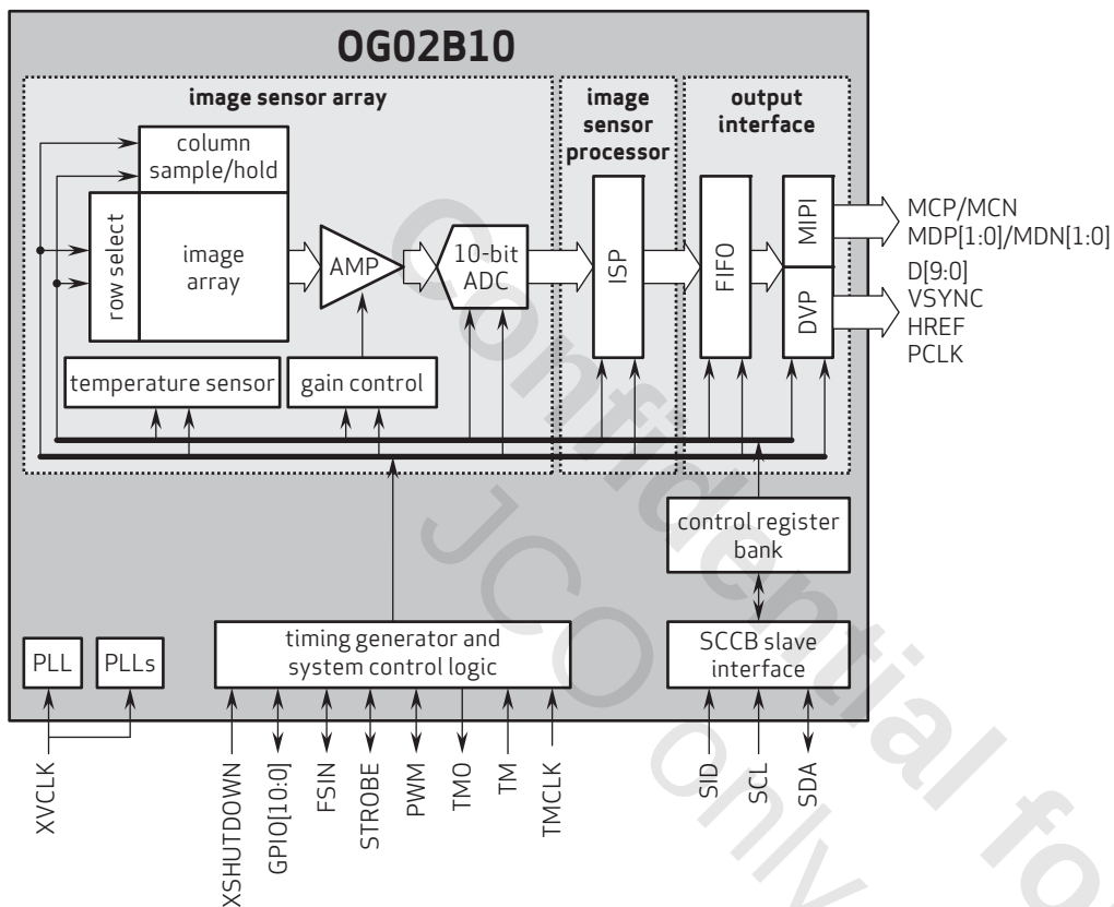
figure 2-1 OG02B10 block diagram
