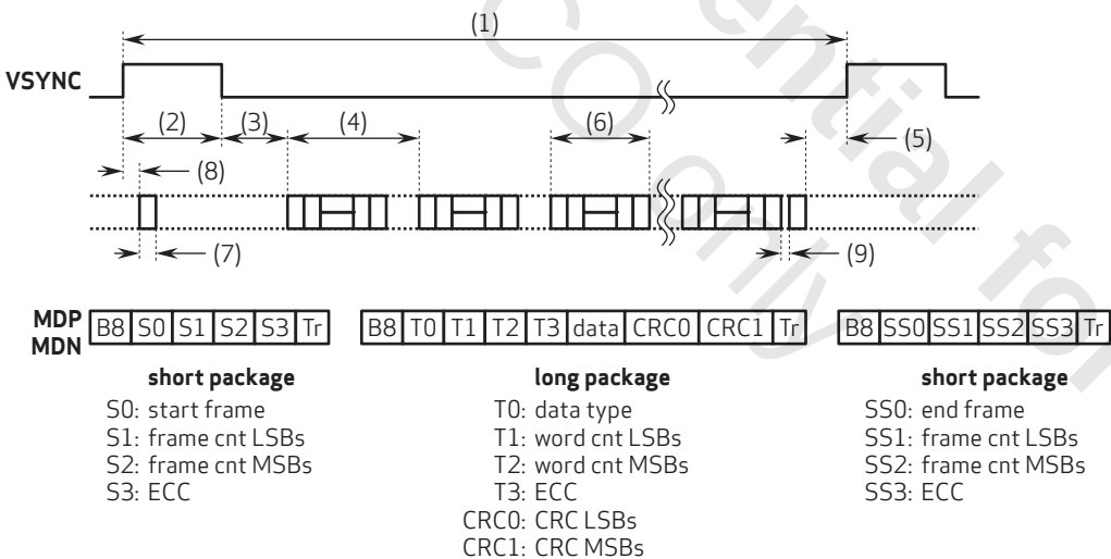
figure 5-1 MIPI timing
