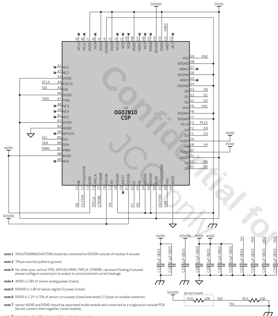
figure 1-3 OG02B10 DVP reference design schematic
